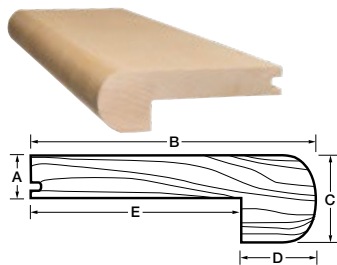
Round edged stair nosing 7/16"
