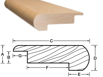
Round edged stair nosing 7/16"
