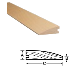
Round reducer 3/8"
