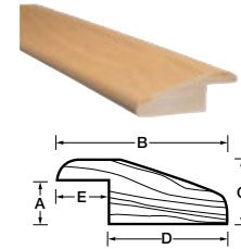
Round reducer 7/16"
