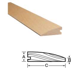
Round reducer 3/8"
