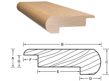
Round Stair Nosing (Floated Installation)
