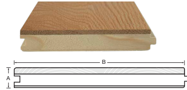
Tread & Riser Planks (Fixed 48" length plank in TruBalance 3/4" board thickness)
