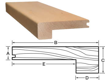
Square edged stair nosing* 1/2"
