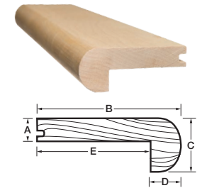
Round edged stair nosing 3/8"
