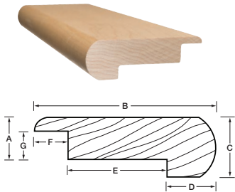
Round Stair Nosing (Floated Installation)
