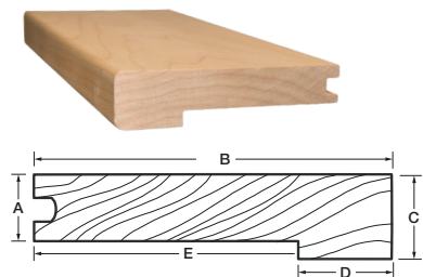
Square edged stair nosing 3/4"
