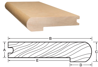
Round edged stair nosing 3/4"
