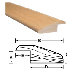
Round reducer 7/16"
